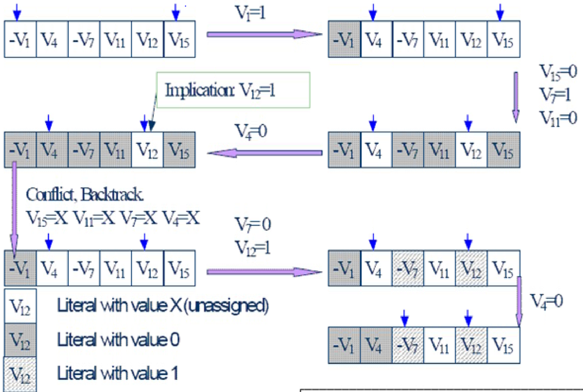
Figure 1: BCP using two watched literals
