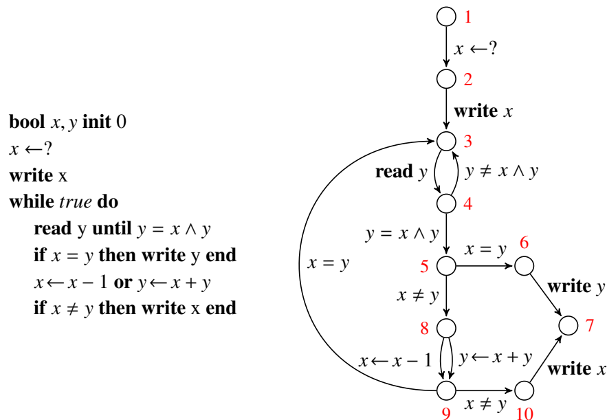
Figure 15.8: Programm used in Exercise 84.
