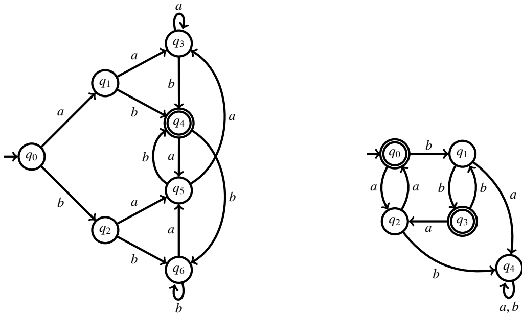
Figure 15.6: DFAs A (left) and B (right) of Exercise 33.
