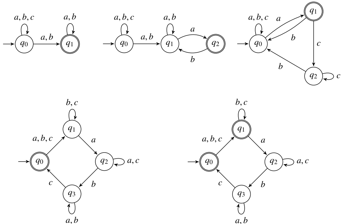
Figure 15.11: Automata for (1)-(5).
