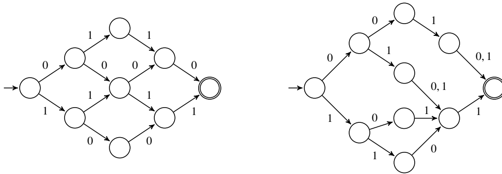
Figure 15.5: DFAs for the languages of Exercise 32.
