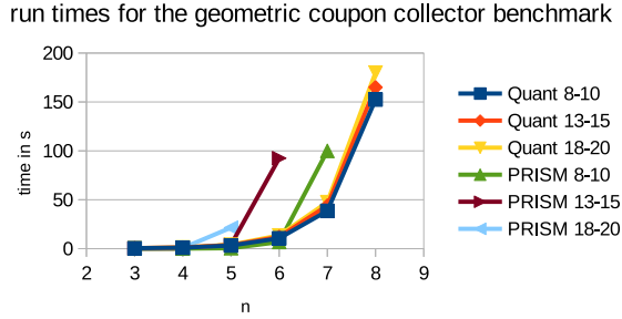
Fig. 4. Run times for the second experiment. Missing data points indicate a timeout or out-of-memory error.
