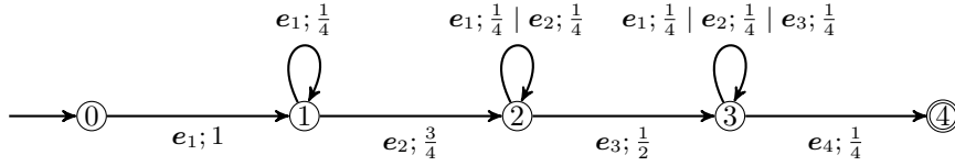
Fig. 1. Cost chain C_n modelling the coupon collector's problem for n = 4 . The loop labelled with e_1; \frac{1}{4} | e_2; \frac{1}{4} represents two loops, labelled with e_1; \frac{1}{4} and e_2; \frac{1}{4} , respectively (and similarly for the right loop).
