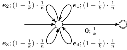
Fig. 2. Cost chain \mathcal{G}_{n,k} modelling the geometric coupon collector's problem for n = 4 .
